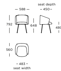
Chair V2 with armrest Tube base
