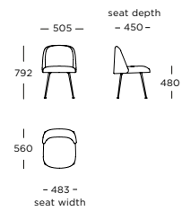
Chair V2 Tube base
